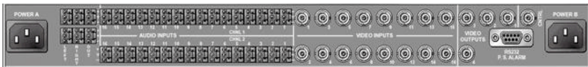
Note: Rear Panel of 16X16 Switcher
